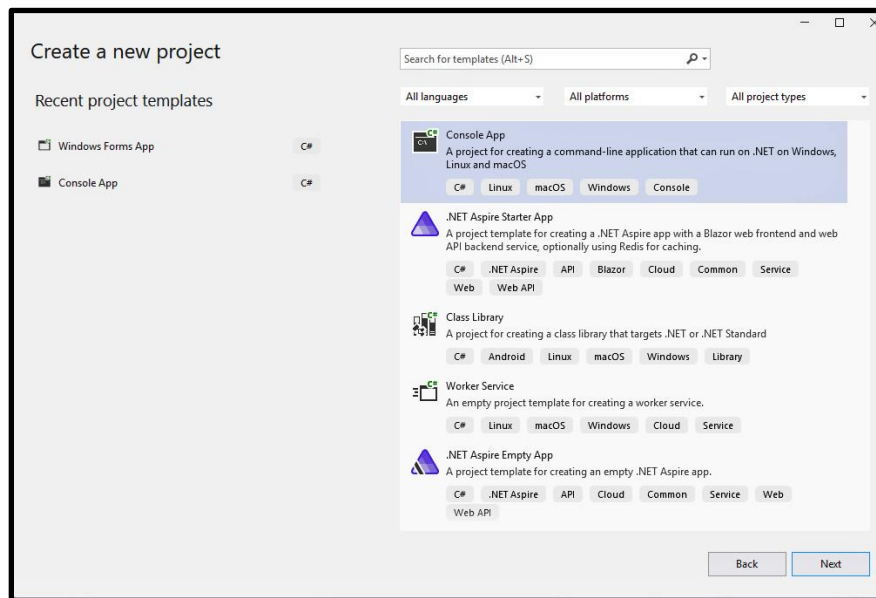
Figure 4.0: Console Application
